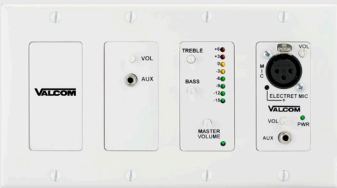
4-Channel Mixer
